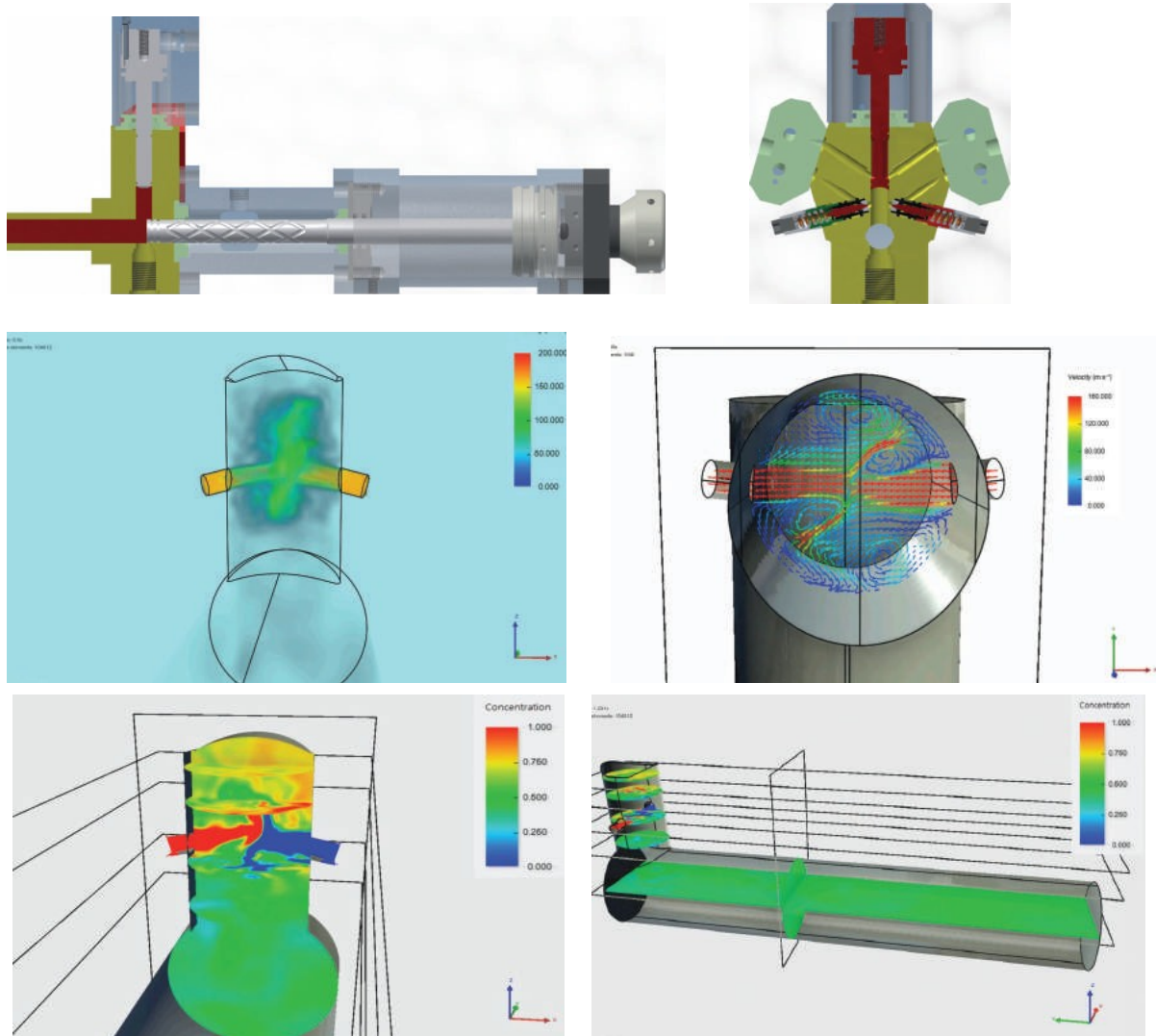
<Flow analysis Red : ISO Blue : POL>
